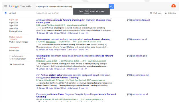
Gambar.1 Searching Literature
